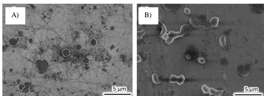
Fig. 4. Microparticles SEM micrographs of 1 % PCL solutions in mixture solvents of Chloroform with acetone or DMF (A) Acetone: Chloroform, 1:3 (v/v), (B) DMF: Chloroform, 1:3 (v/v) with electro spray parameters voltage: 18 kV, collecting distance: 18 cm, flow rate: 1 ml/h, gauge 20G
